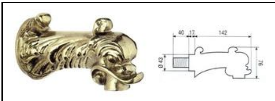
Art. 930 ¾ “ F connection continuous fountain supplier
